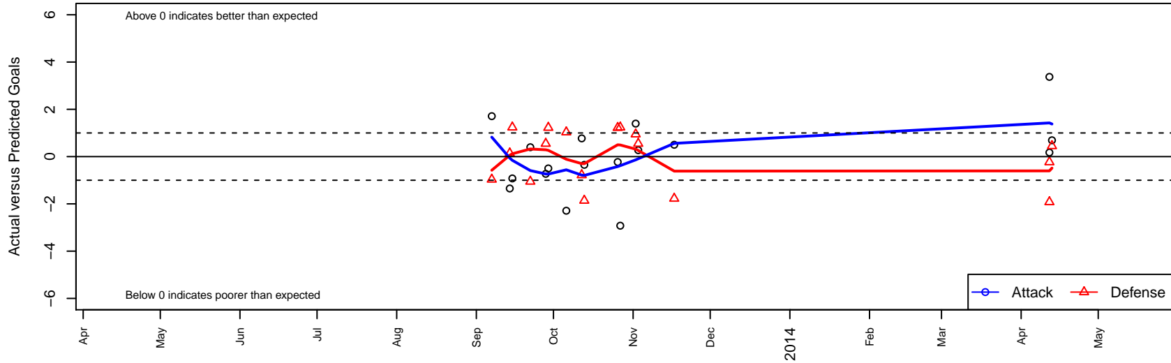
FC Golden State Black B96 Dots are actual minus expected GF (blue circles) and GA (red triangles). Blue line is smoothed change in attack strength. Red is smoothed change in defense strength.
